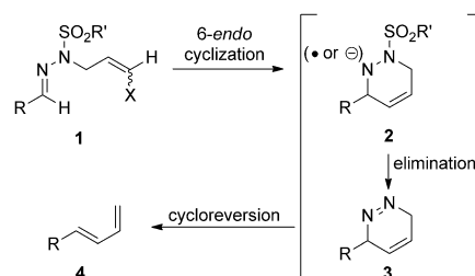
Scheme 1. Proposed route to dienes from hydrazones.
